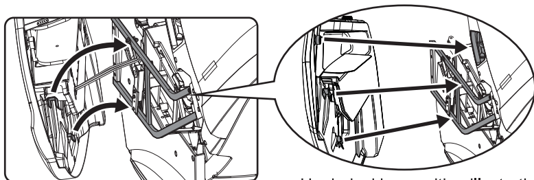
Hook docking position illustration
